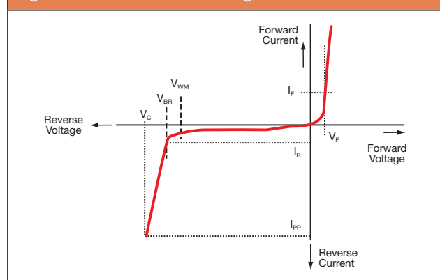
Figure 3. Parameters of voltage and current
