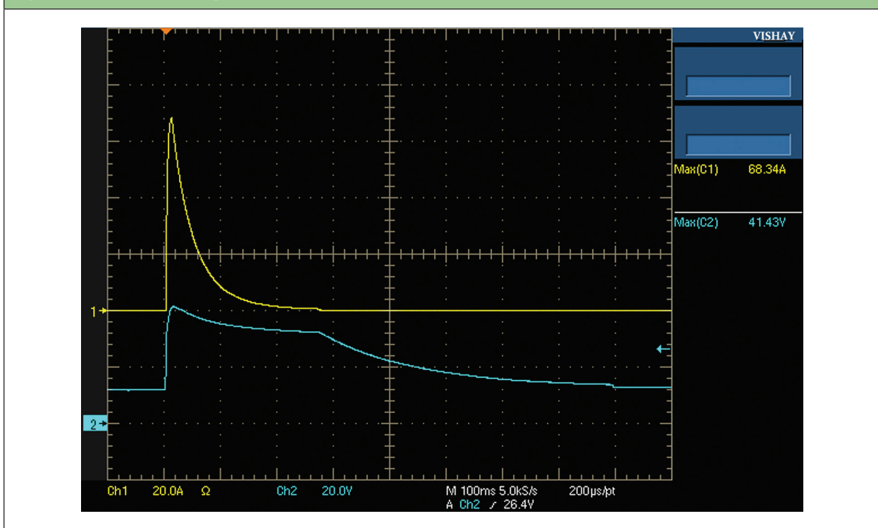
Figure 7a: Clamped voltage and current of SM5S24A in ISO 7637-2 test
