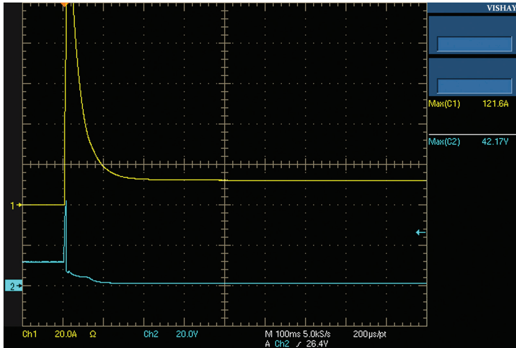
Figure 7b: Clamped voltage and current of load dump TVS failures in ISO7637-2 test
