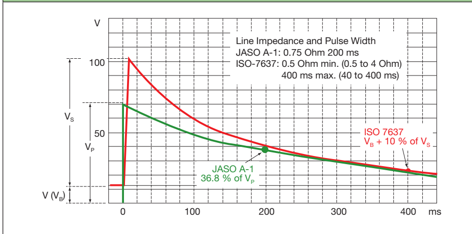
Figure 6. For ISO-7637-2 test conditions, the standard condition is a V_S range of 65 V to 87 V, and R_i (line impedance) range of 0.5 \Omega to 4 \Omega
