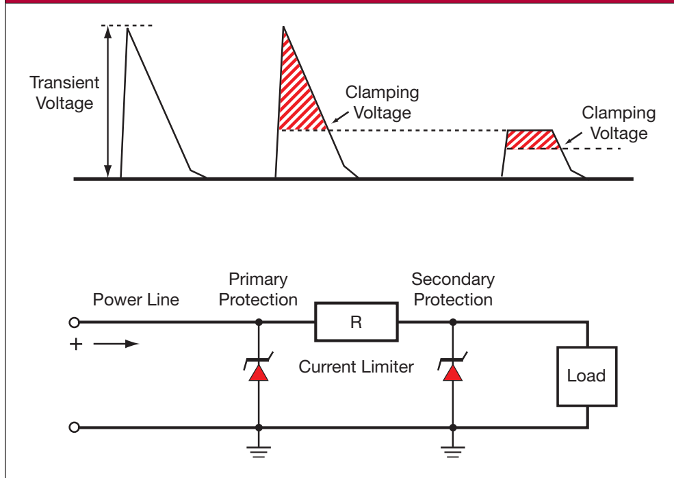
Figure 9. Secondary protection circuit
