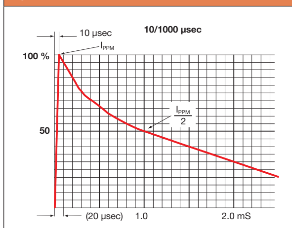
Figure 1. Test waveform of TVS
