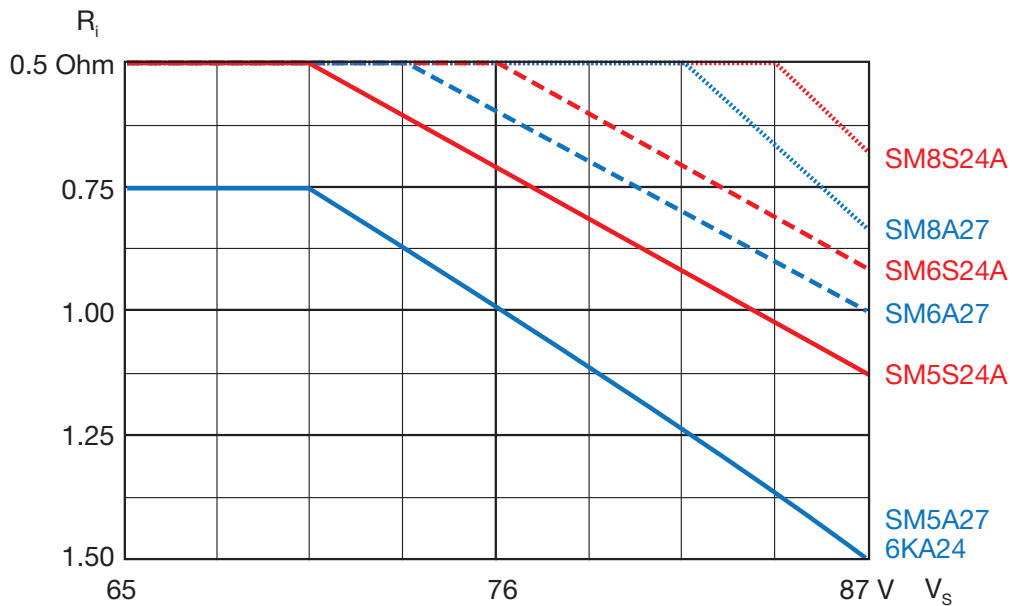
Figure 7c: Maximum clamping capability of Vishay load dump TVS in ISO7637-2 test
